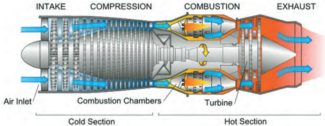
Fig 34: Gas turbine
