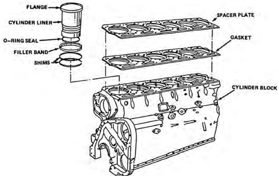
Fig 28: Cylinder
